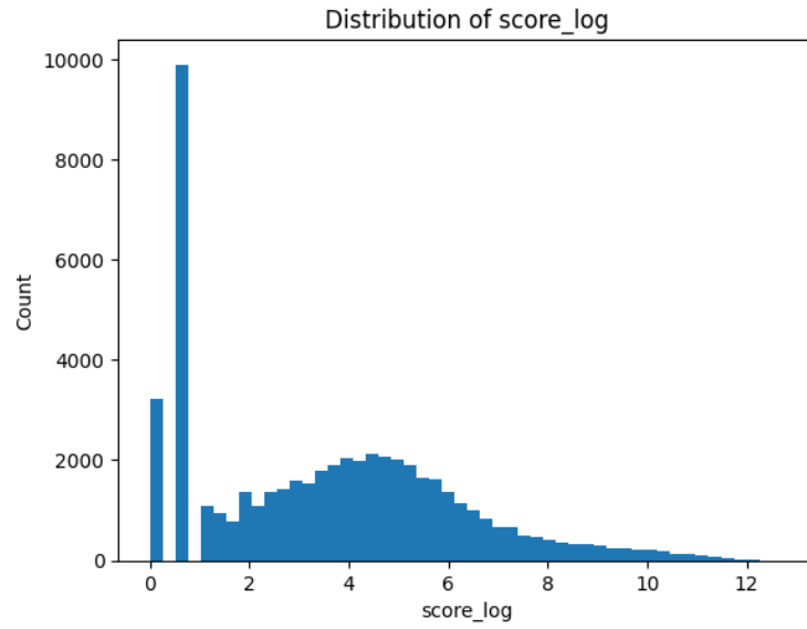
Figure A.25. Log-transformed score distribution ( \text{score\_log} = \log_{10}(\text{score}) ) approximating a bell shape.
